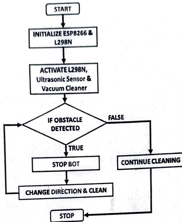
Figure 2. System Flowchart
